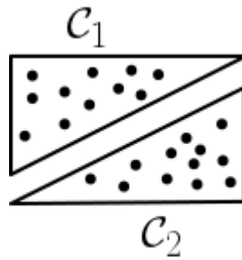
FIGURE 2. Set of data points uniformly distributed within two right angled triangles forming classes \mathcal{C}_1 and \mathcal{C}_2 .
